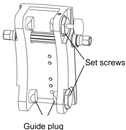
Slider with sliding guide
