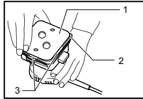
1. Punch plate 2. Sandpaper 3. Guide
